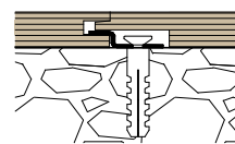
Installazione pannelli successivi Boiserie-V Installation of following panels Boiserie-V
