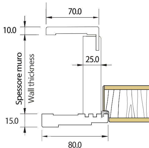
Quote stipite / Jamb dimensions
