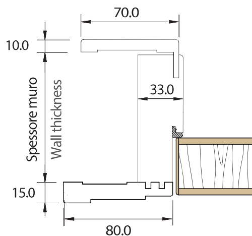
Quote stipite / Jamb dimensions
