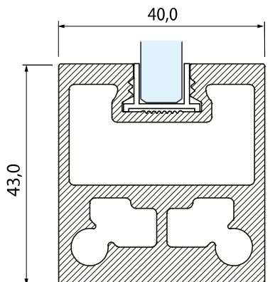
TRAVERSO / Beam
